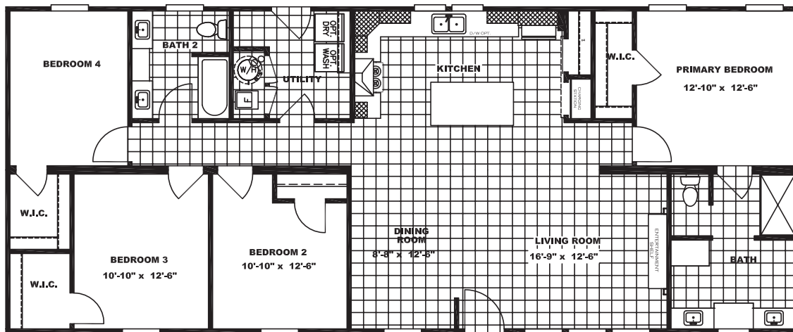
OPT. WALK-IN SHOWER BATH
